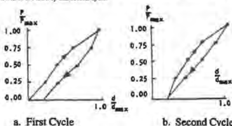
Figure 1. Static Load Test Load-Deflection Curves
